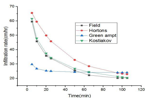
Figure 3: Comparison of infiltration rate
